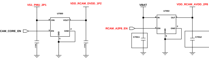
RCAM1 LDO
