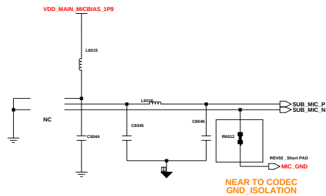
Sub MIC NC
