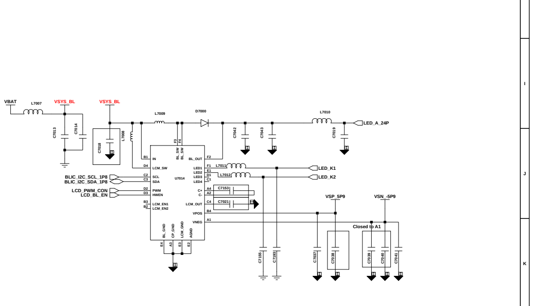
CAMERA MIPI SWITCH LCD_LDO BLIC Engineer: CAMERA, DISPLAY Drawn by: R&D CHK: TITLE: Size: DOC CTRL CHK: SM-A02 MFG ENGR CHK: Changed by: Date Changed: Time Changed: QA CHK: REV Drawing Number: Page: 7/7 2 3 4 5 6 7 8 9 10 11 12 13 14 15 16
