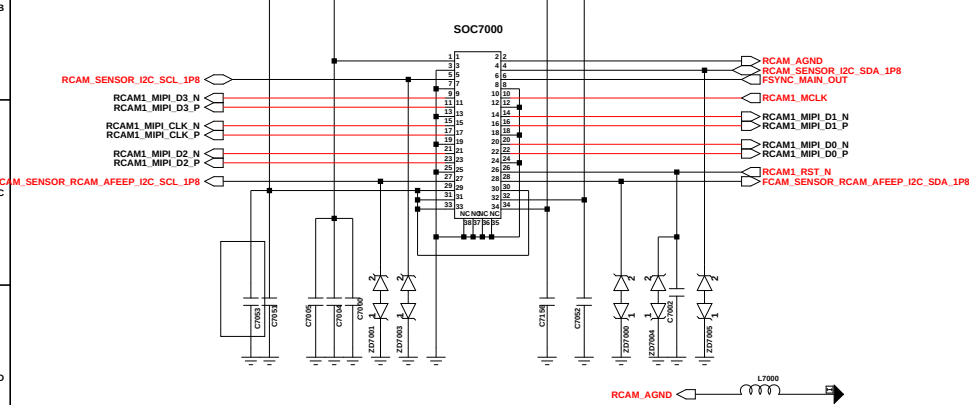
RCAM1_13M_34pin
